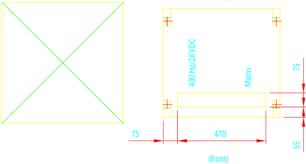
Foundation plan
