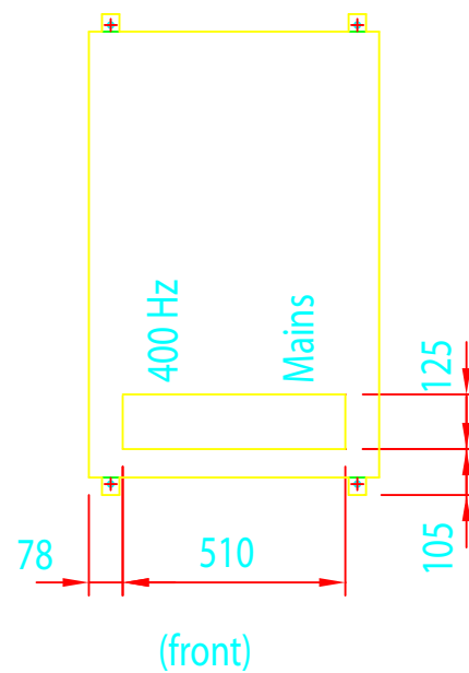
Foundation plan
